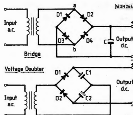
Fig. 5.6: Full wave, bridge and voltage doubler rectifier circuits
