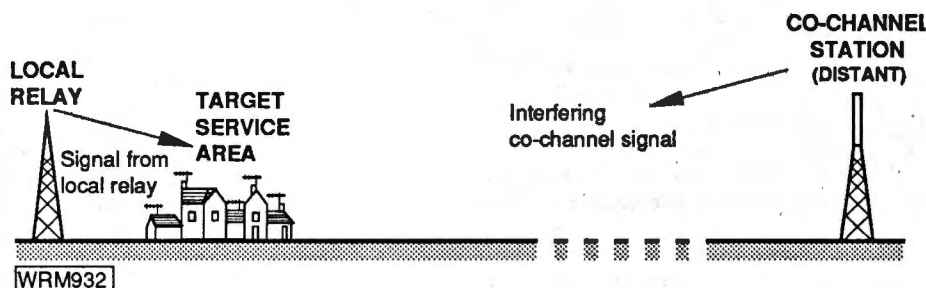
Fig. 8.3: Correct siting of a relay station reduces the effects of co-channel interference by making use of the radiation pattern of the receiving antenna
