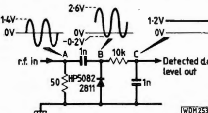
Fig. 2: Simple but inefficient r.f. detector circuit
